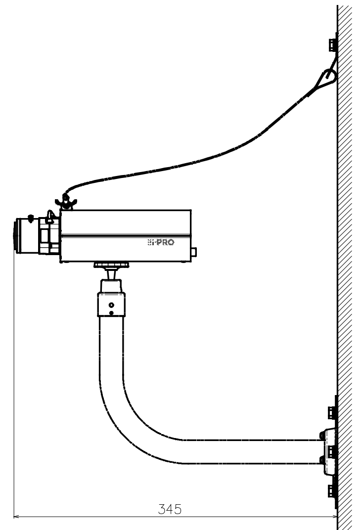
Attach to WV-Q181UX (S=1:2)
