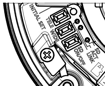
Detail B (2:1)
