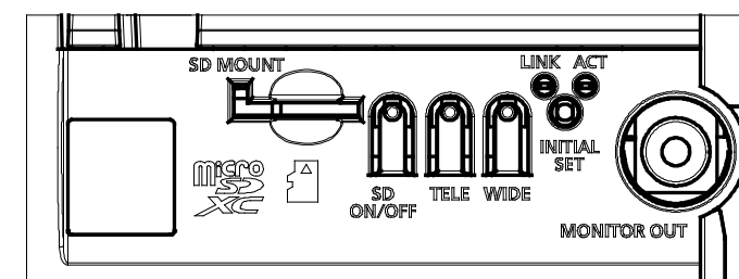
Detail A (2:1)
