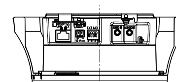
Inside of Decorative cover (lower part)
