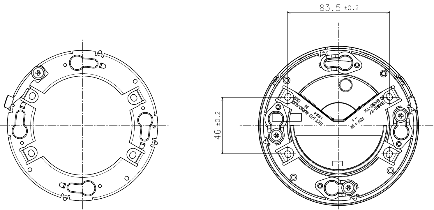
Attachment plate
