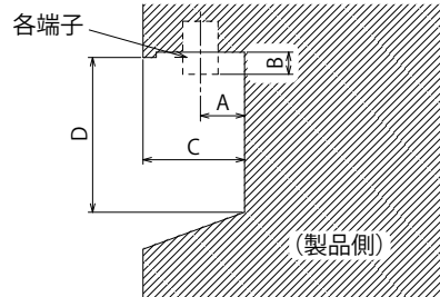
端子部 b 断面 (IR OUT/SERIAL IN/OUT/AUDIO OUT/IR IN/AV IN)
