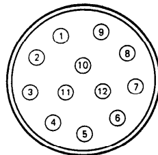
HR10A-10TP-12S
