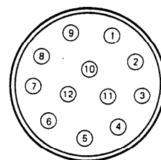
HR10A-10TP-12P
