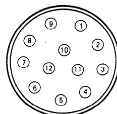
HR10A-10TP-12P
